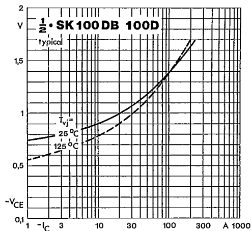
Fig. 11 Inverse diode forward characteristics
